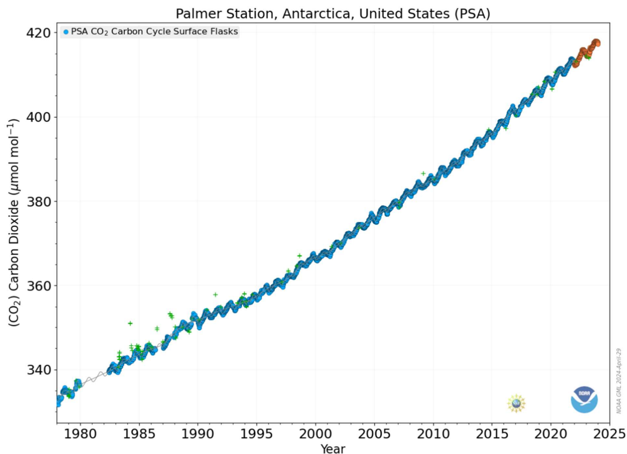
Figure 5. Carbon Dioxide ( \text{CO}_2 ) levels at Palmer Station dating back to 1980. Orange dots are preliminary data and green pluses are poorly mixed air masses, which should not indicate background conditions.
