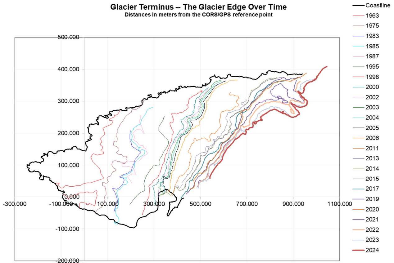
Figure 9: 61 Years of Glacier Retreat Data
