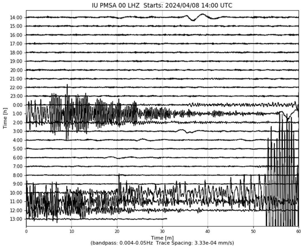
Figure 3. The April 9th 6.6 earthquake in the Molucca Sea, as recorded from the Palmer seismic station.
