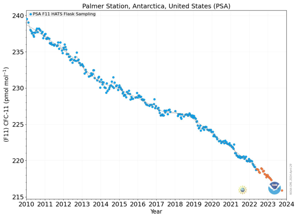
Figure 6. Chlorofluorocarbon-11 (CFC-11) levels at Palmer Station dating back to 2010, one of the Halocarbon and Trace Gases measured at Palmer Station. Orange dots are preliminary data.
