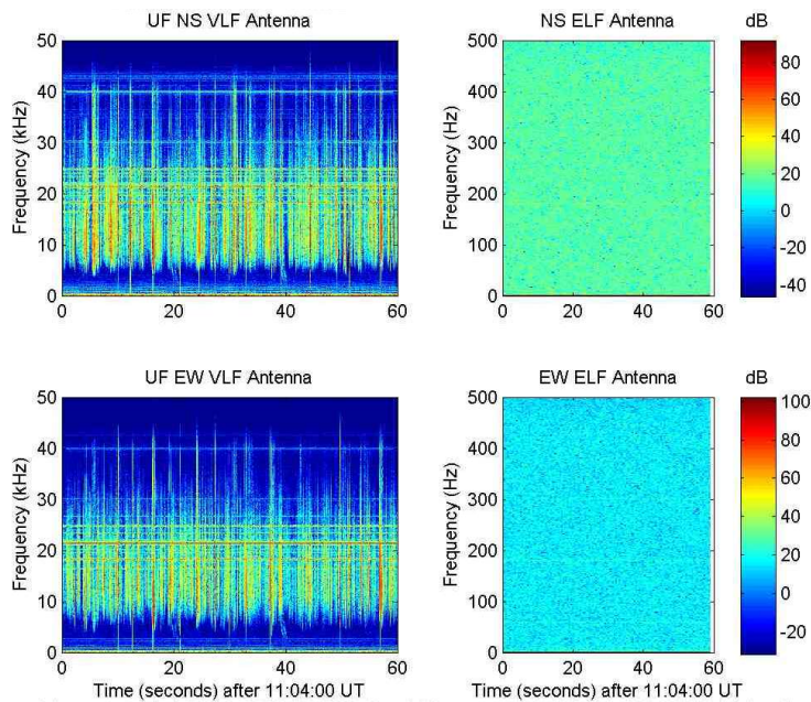
Figure 2. Real-Time broadband VLF and ELF Spectrogram from Palmer Station, Antarctica.
